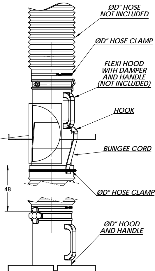
FRONT VIEW
