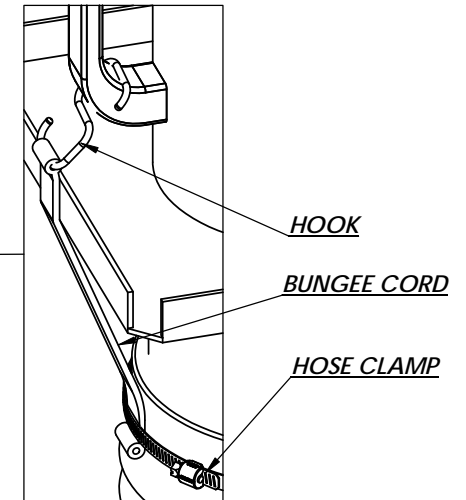
DETAIL VIEW
