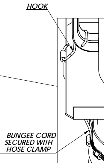
DETAIL VIEW #1
