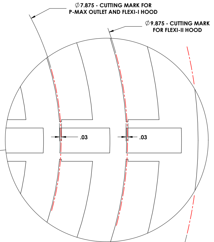
DETAIL VIEW
