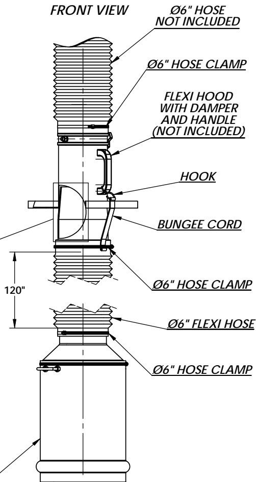
RCA NOZZLE
