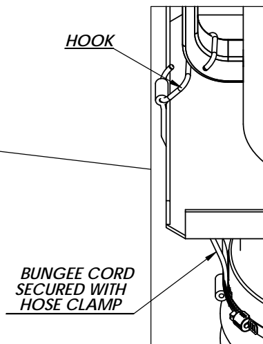
DETAIL VIEW
